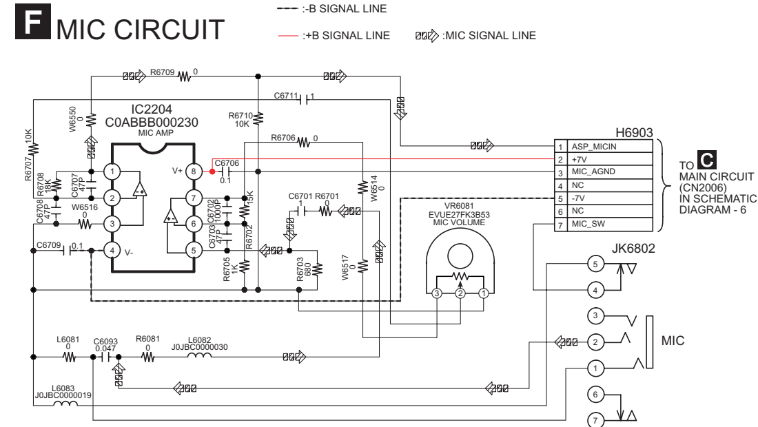
SCHEMATIC DIAGRAM - 10
